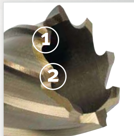
Heavy duty serration with pre- (1) and post-cutter (2)
